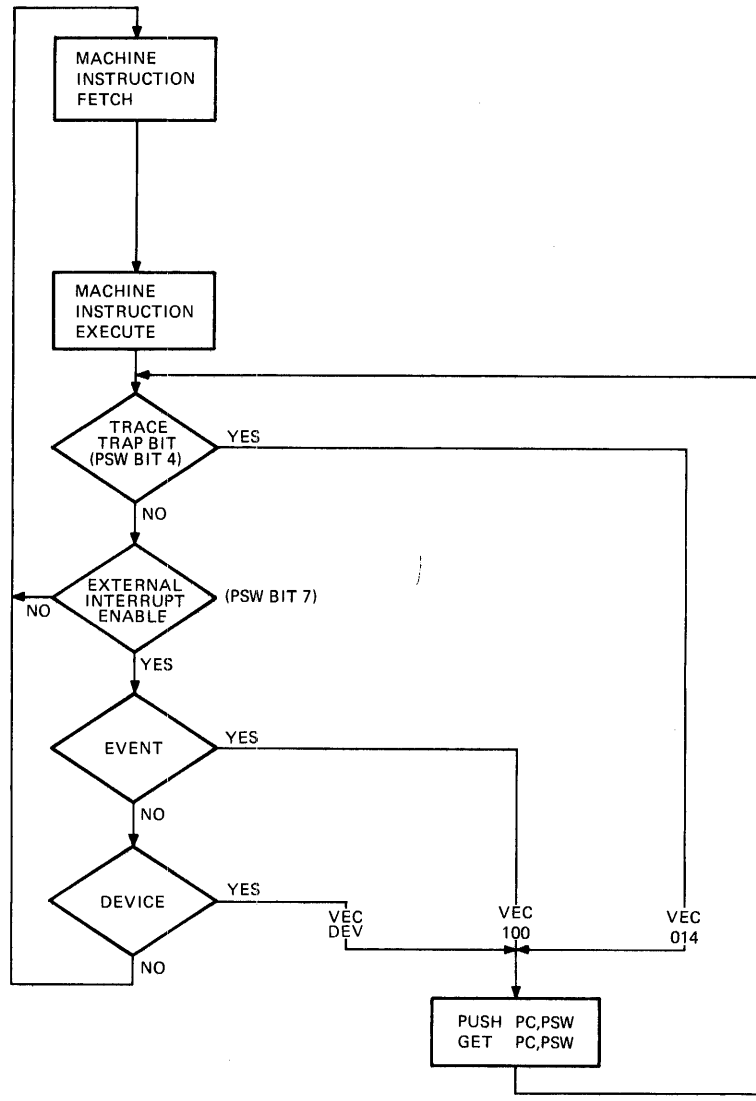
Interrupt and Trap Portion of Machine Cycle Figure 2-15
